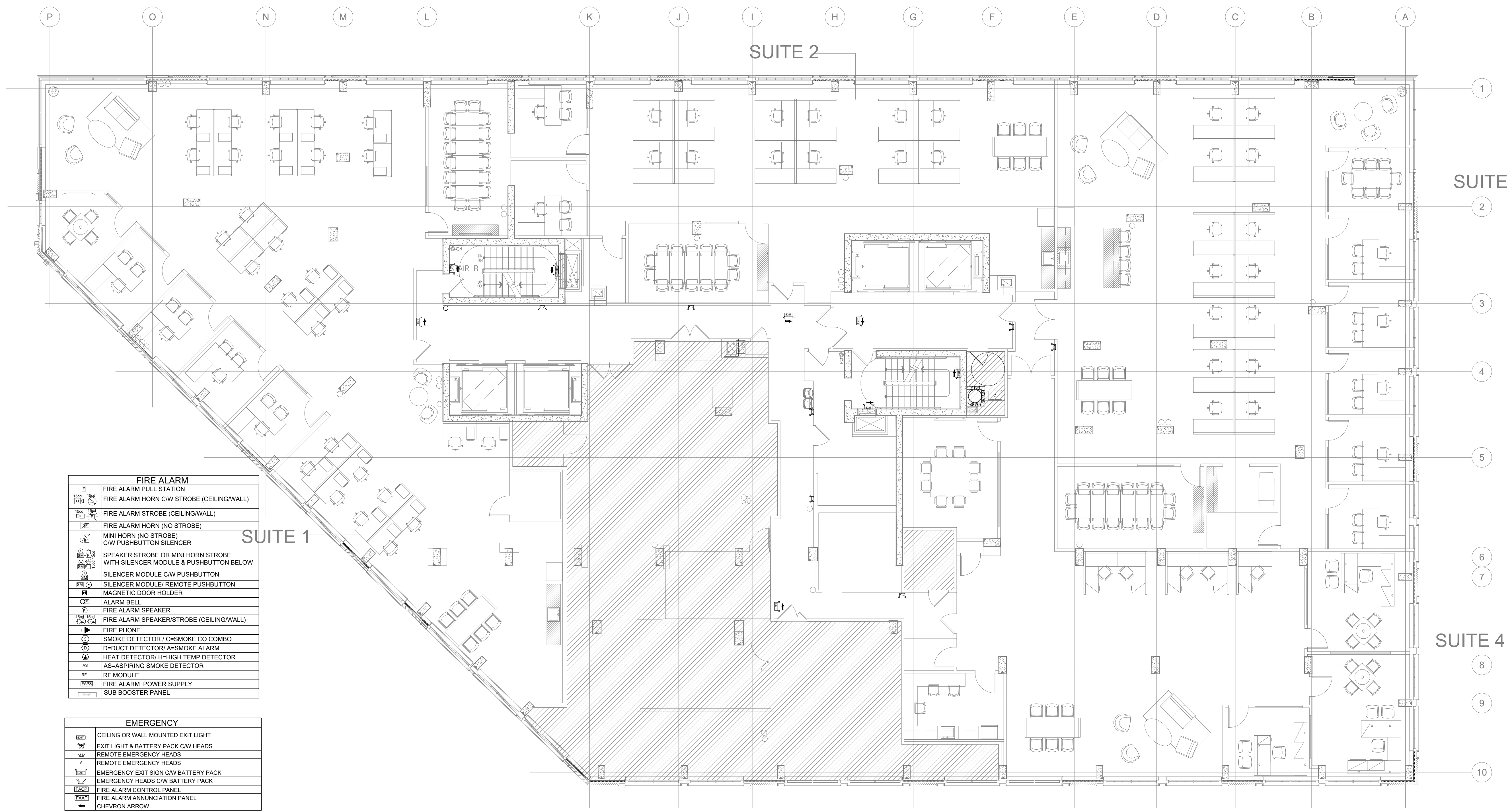
1 A-2.0 EMERTGENCY LIGHTING 7TH FLOOR PLAN SCALE: 3/4" = 1'-0" GROUND LEVEL
