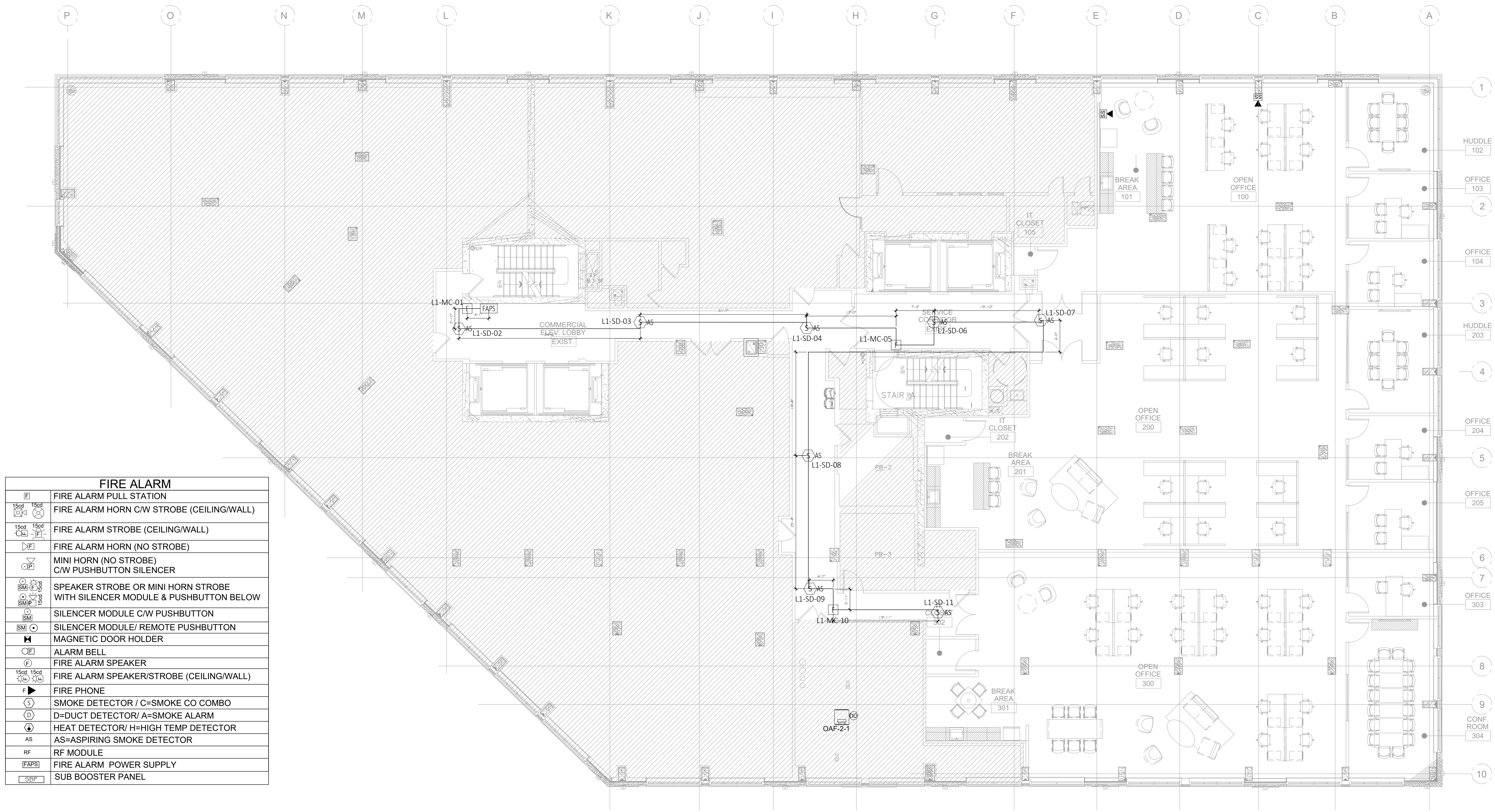
FIRE ALARM 2ND FLOOR PLAN SCALE: 3/8" = 1'-0" GROUND LEVEL
