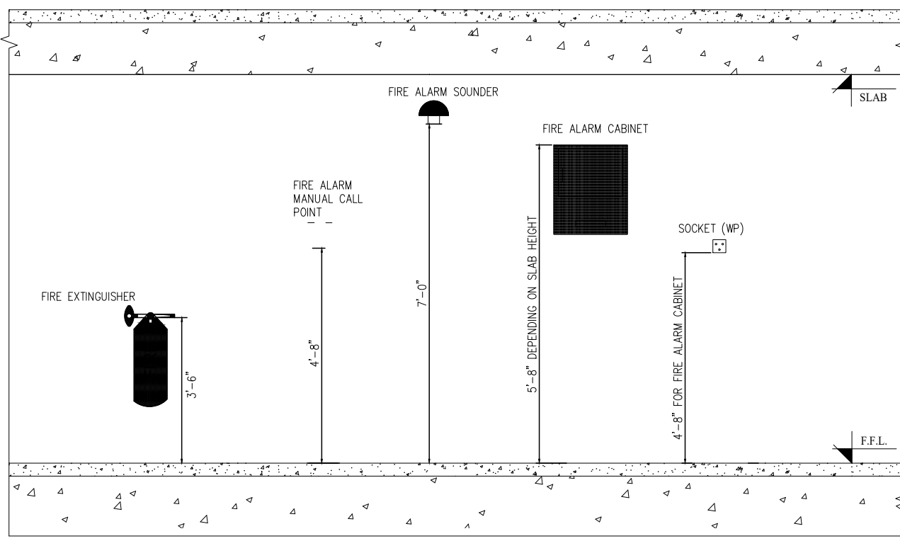
10 EL STANDARD MOUNTING HEIGHT OF FIRE ALARM ACCESSORIES SCALE : N.T.S
